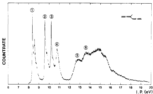
Figure 2. PE spectrum of 3-methyl-1,2,4,5-hexatetraene (3-methylbiallyl, 2 ).
