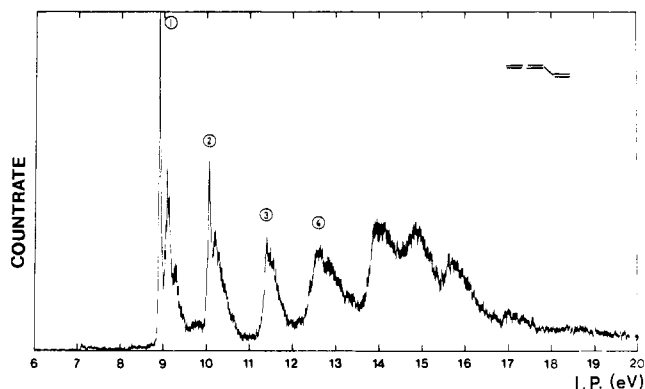
Figure 4. PE spectrum of 1,2,4-pentatriene (vinylallene, 3).
