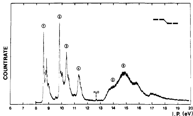
Figure 1. PE spectrum of 1,2,4,5-hexatetraene (biallenyl, 1 ).
