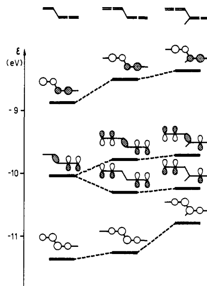
Figure 3. Comparison between the first bands of the PE spectra of 1 , 2 , and 3 .
