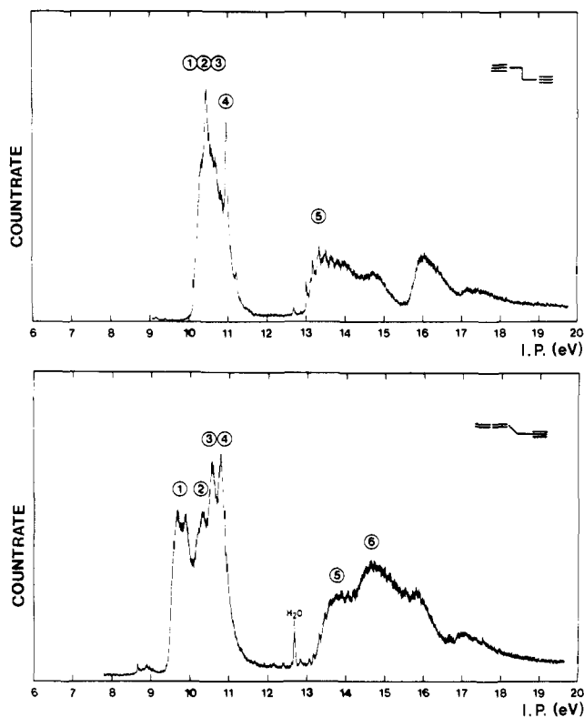
Figure 6. PE spectra of 1,2-hexadiene-5-yne (propargyllene, 4 ) and 1,5-hexadiyne (bipargyl, 5 ).
