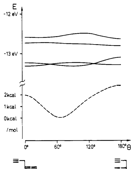
Figure 5. Highest four occupied MO's of 4 as a function of \theta (top) and total energy of 4 as function of \theta (bottom) according to an EH calculation.
