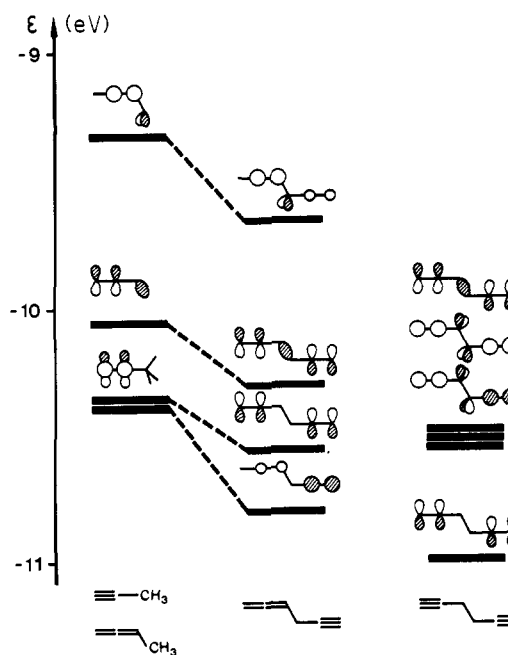
Figure 7. Comparison between the first bands of the PE spectra of methylallene and methylacetylene (left) with those of 4 (middle) and 5 (right).
